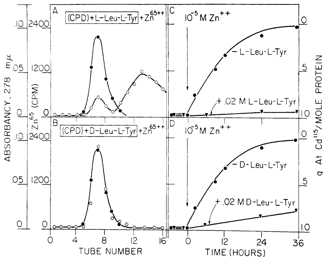
FIG. 7.—A and B, prevention of Zn 65++ binding to apocarboxypeptidase, (CPD), by L-leucyl-L-tyrosine (L-Leu-L-Tyr) and binding of Zn 65++ to apocarboxypeptidase in the presence of D-leucyl-L-tyrosine (D-Leu-L-Tyr). One ml samples of 5 \times 10^{-6} M (CPD) plus 2 \times 10^{-2} M L-Leu-L-Tyr plus 5 \times 10^{-6} M Zn 65++ (A); and 5 \times 10^{-6} M (CPD) plus 2 \times 10^{-2} M D-Leu-L-Tyr plus 5 \times 10^{-6} M Zn 65++ (B) were passed over a 1 \times 30 cm, G-25 Sephadex column at a flow rate of 1 ml per minute. Absorbancy at 278 mμ (●) and Zn 65++ (○), counts per minute per 2 ml fraction were determined on successive 2 ml fractions. Conditions of preincubation as in Fig. 1B. C and D, exchange of Zn ++ for cadmium 115 in [(CPD)Cd 115 ] in the presence (+) and absence (—) of L-Leu-L-Tyr and D-Leu-L-Tyr. As controls, 1 \times 10^{-6} M [(CPD)Cd 115 ] was exposed to 1 \times 10^{-5} M stable Zn ++ at 0 time and the Cd 115++ bound to the enzyme (●) measured as dialysis progressed. 1 \times 10^{-6} M [(CPD)Cd 115 ] was equilibrated for 2 hours with 2 \times 10^{-2} M L-Leu-L-Tyr (C) or 2 \times 10^{-2} M D-Leu-L-Tyr (D) followed by the addition of 1 \times 10^{-5} M Zn ++ at 0 time. Cd 115++ bound to the enzyme (▼) was measured as dialysis progressed.
