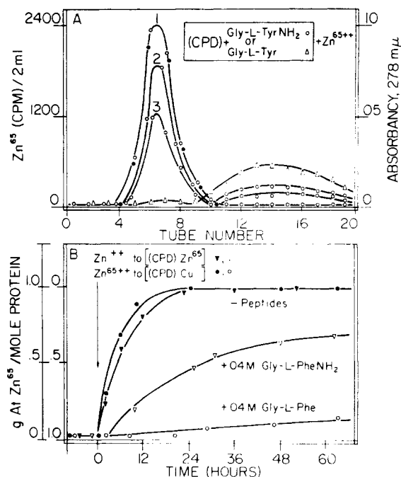
FIG. 8.—A, prevention of Zn^{65++} binding to apocarboxypeptidase, (CPD), by glycyl-L-tyrosine amide (Gly-L-TyrNH 2 ) and glycyl-L-tyrosine (Gly-L-Tyr). One ml of (CPD), 5 \times 10^{-6} M, plus Zn^{65++} , 5 \times 10^{-6} M, is the control (curve 1). The same concentration of (CPD) was exposed to Gly-L-TyrNH 2 , 0.05 M (curve 2) and 0.1 M (curve 3), and then to Zn^{65++} , 5 \times 10^{-6} M. (CPD), 5 \times 10^{-6} M, was also exposed to Gly-L-Tyr, 0.05 M, followed by the addition of Zn^{65++} , 5 \times 10^{-6} M. All samples were passed over a 1 \times 30 cm, G-25 Sephadex column and absorbancy at 278 mμ (●) and Zn^{65++} in the presence of Gly-L-TyrNH 2 (○) or Gly-L-Tyr (Δ), counts per minute per 2 ml fraction, were determined on successive 2 ml fractions. Absorbancy at 278 mμ, similar in all experiments, is plotted only for the control. Conditions of preincubation as in Fig. 1B. B, exchange of Zn^{65++} for zinc 65 in [(CPD)Zn 65 ] or Zn^{65++} for copper in [(CPD)Cu] in the presence (+) and absence (—) of Gly-L-PheNH 2 and Gly-L-Phe. As controls, 1 \times 10^{-5} M [(CPD)Zn 65 ] was exposed to 1 \times 10^{-5} M Zn^{65++} or 1 \times 10^{-5} M [(CPD)Cu] was exposed to 1 \times 10^{-5} M Zn^{65++} at 0 time, and the Zn^{65++} either remaining bound (▼) or being bound (●) by the enzyme was measured as dialysis progressed. Experiments in the presence of Gly-L-PheNH 2 (▽) and Gly-L-Phe (○) were conducted under identical conditions.
